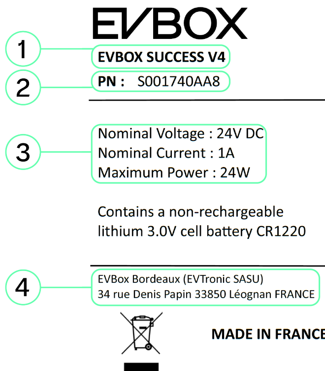
EVBox Success nameplate
