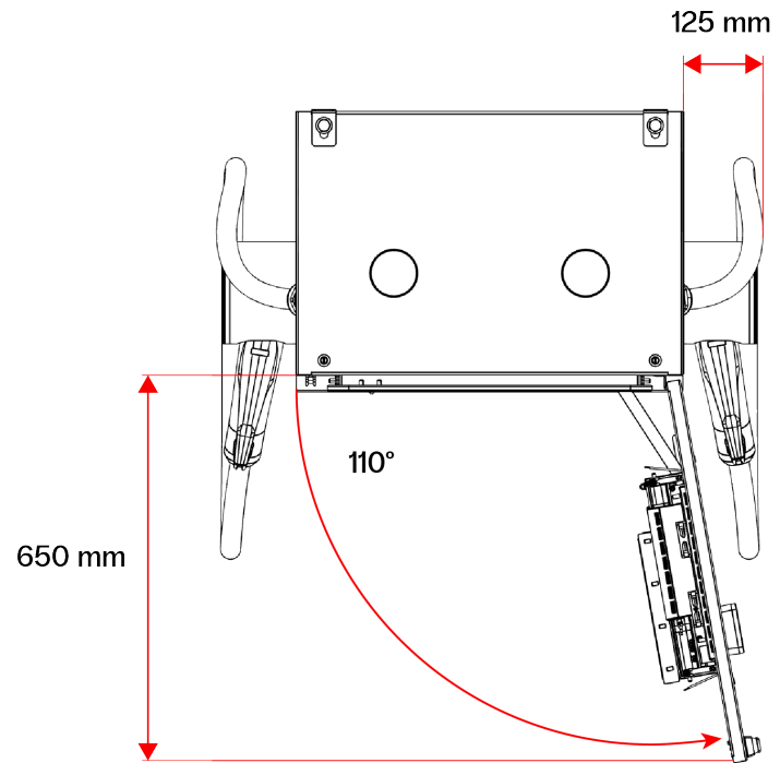
Troniq Compact Modular overall dimensions
